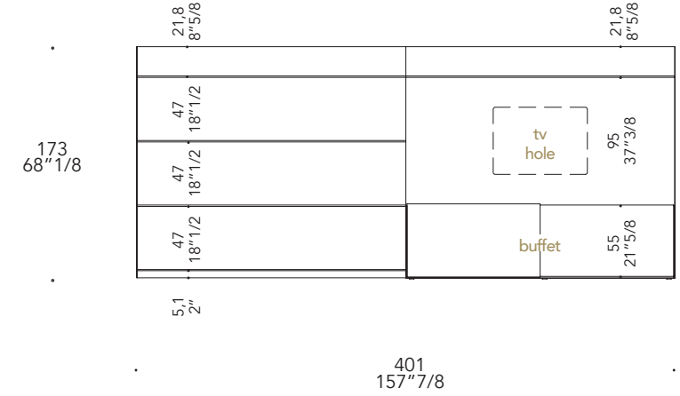
COMPOSITION 3 Boiserie panels + shelves + buffet + boiserie TV
